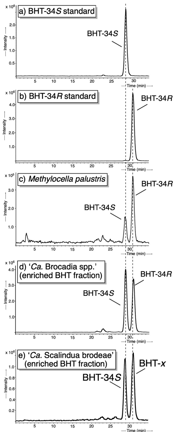
Fig. 4. HPLC-MS mass chromatograms ( m/z 655) of acetylated a) BHT-34S standard; b) BHT-34R standard; c) BDE of Methylocella palustris ; d) BDE ' Ca. Brocadia sp.'; e) BDE from ' Ca. Scalindua brodeae '.
