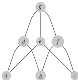
Figure 2.2 Examples of structures that all have a unique sum
