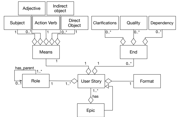
Fig. 2. Conceptual model of user stories
