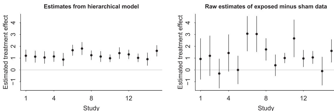
FIGURE 6 A, Posterior mean ± SD of each treatment effect \theta_j from the hierarchical model fit to the repeated transcranial magnetic stimulation data. The fitted model did not estimate the sham effects to be zero, and so these estimated treatment effects take into account both the exposed and sham data. B, For comparison, the raw difference estimates y_{j1} - y_{j0} \pm standard error. The Bayesian hierarchical estimates on the left plot are partially pooled toward a common mean
