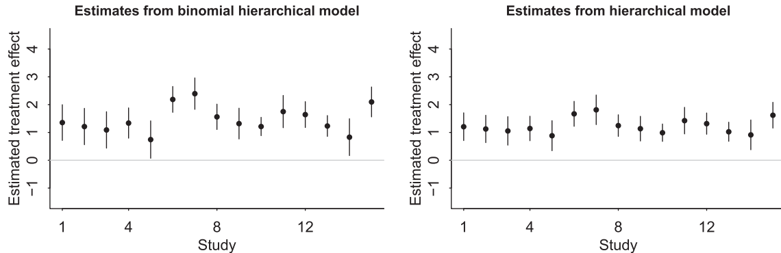
FIGURE D1 A, Posterior mean \pm SD of each treatment effect \theta_j from the hierarchical model (D1) with binomial likelihood. B, For comparison, the same estimates from the hierarchical model (2) with normal likelihood
