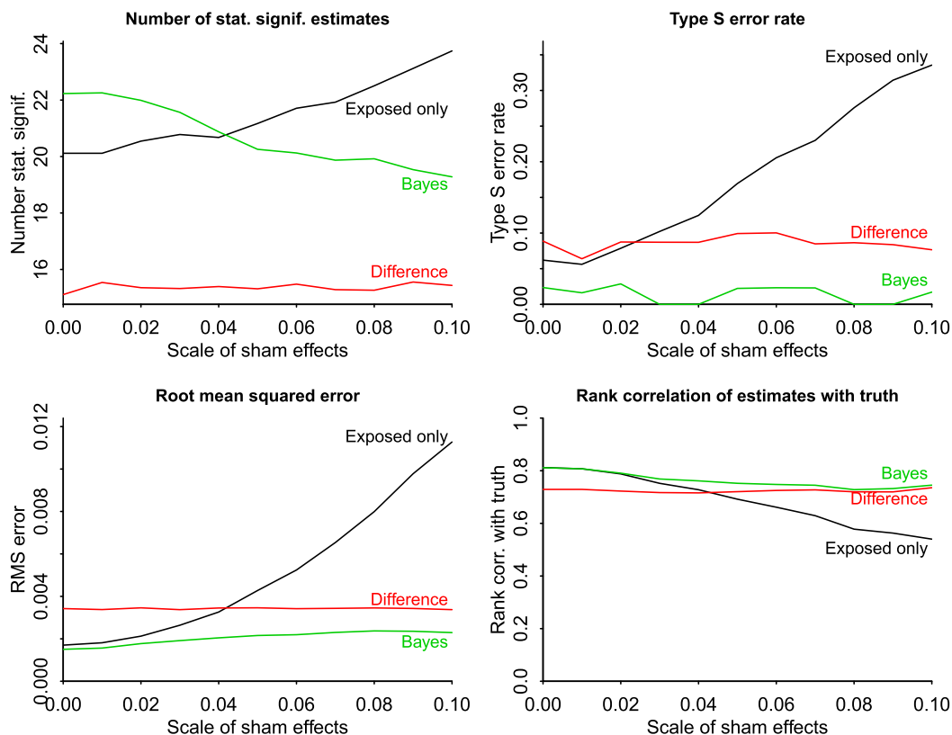
FIGURE B1 Results of the alternative simulation study from Appendix B1 comparing three estimates—the exposed data estimate, y_{j1} , the difference between exposed and sham, y_{j1} - y_{j0} , and the Bayesian hierarchical model estimate E(\theta_j|y) —to simulated data. The four graphs show the results for four different frequency evaluations, and on each graph the horizontal axis represents \sigma^b , the SD of the sham effects in the simulation [Colour figure can be viewed at wileyonlinelibrary.com ]
