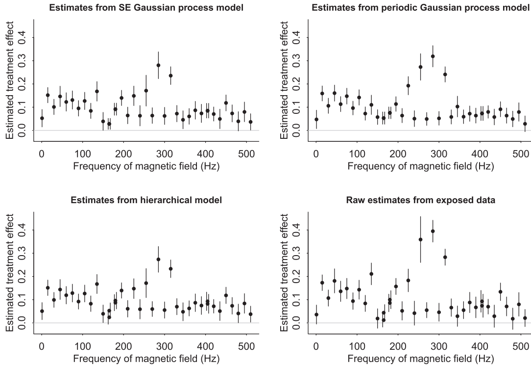
FIGURE A2 Top row: A, Posterior mean \pm SD of each treatment effect \theta_j from the squared-exponential kernel Gaussian process model fit to the chick data. B, The corresponding plot for the periodic kernel Gaussian process model. The fitted models estimate the sham effects to be essentially zero, and so these estimated treatment effects come pretty much from the exposed data alone. The Bayesian estimates in the left plot are partially pooled toward each other for close frequencies. The estimates in the right plot are partially pooled toward each other for frequencies whose difference is close to 30 Hz. Bottom row: For comparison, C, the estimates from our default analysis and D, the raw estimates y_{j1} from the exposed data
