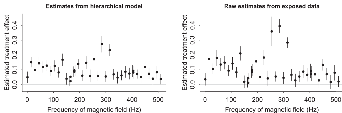
FIGURE 3 A, Posterior mean \pm SD of each treatment effect \theta_j from the hierarchical model fit to the chick data. The fitted model estimated the sham effects to be essentially zero (see discussion of Table 2), and so these estimated treatment effects come pretty much from the exposed data alone. For three of the frequencies (165, 180, and 405 Hz) the experiment was performed twice, and in these cases we have jittered the two experimental results so they both appear on the graph. B, For comparison, the raw estimates y_{j1} \pm standard error. The Bayesian hierarchical estimates on the left plot are partially pooled toward a common mean
