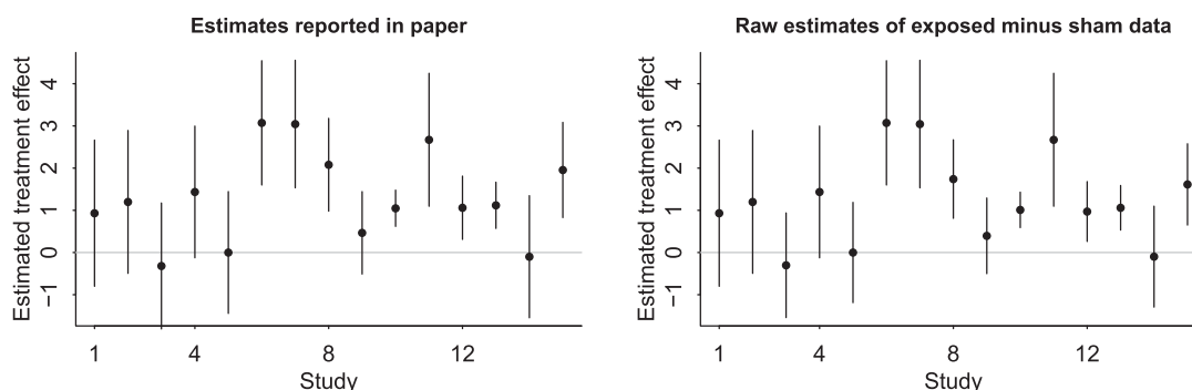
FIGURE 4 A, Estimated effects for each of the repeated transcranial magnetic stimulation experiments as reported by Berlim et al. 6 B, Raw difference estimates y_{j1} - y_{j0} with standard errors (s_{j1}^2 + s_{j0}^2)^{1/2}
