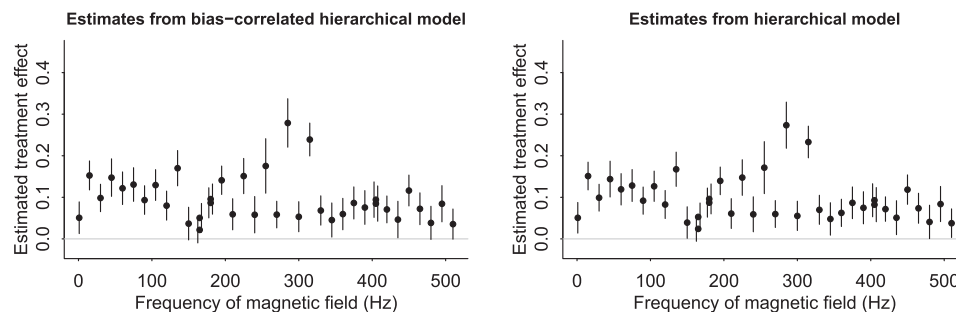
FIGURE A1 A, Posterior mean \pm SD of each treatment effect \theta_j from the hierarchical model with correlated bias and treatment effects fit to the chick data. B, For comparison, the estimates of the original hierarchical model without correlations, which can be seen to be almost identical
