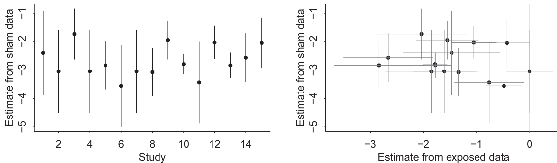
FIGURE 5 A, Estimates ± standard errors of the effect of the sham treatments for the studies in the meta-analysis of repeated transcranial magnetic stimulation. B, Sham vs exposed estimates
