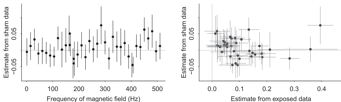
FIGURE 2 A, Estimates \pm standard errors of the effect of the sham treatment as a function of frequency of the (turned off) electromagnetic field; B, Sham vs exposed estimates. Unsurprisingly, given the careful design of the experiment, there is no evidence that the sham effects are anything other than zero
