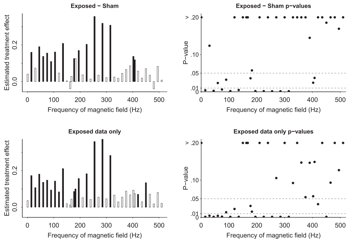
FIGURE 1 Top row: Redrawn versions of the graphs of Blackman et al., 17 summarizing the chick brains data by categorizing estimates at different frequencies based on their statistical significance: A, Estimates y_{j1} - y_{j0} plotted vs frequencies x_j . For three of the frequencies (165, 180, and 405 Hz) the experiment was performed twice, and in these cases we have jittered the two experimental results so they both appear on the graph. Each bar is shaded if the experimental result is statistically significant at the 5% level based on the appropriate t distribution. B, Results of each experiment displayed as a P -value. Bottom row: Corresponding plots using only the exposed data, y_{j1} . The patterns are similar but with enough differences to change some of the reported results
