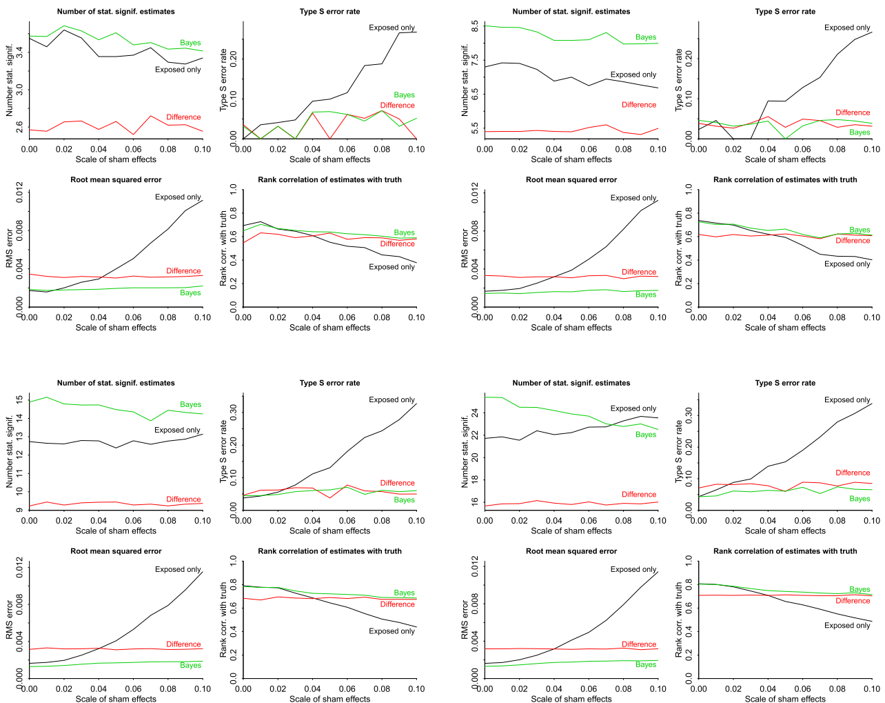
FIGURE C1 Results of simulation studies for datasets of sizes 5 (top left), 10 (top right), 20 (bottom left), and 38 (bottom right), comparing three estimates—the exposed data estimate, y_{j1} , the difference between exposed and sham, y_{j1} - y_{j0} , and the Bayesian hierarchical model estimate E(\theta_j|y) —to simulated data. The four graphs show the results for four different frequency evaluations, and on each graph the horizontal axis represents \sigma^b , the SD of the sham effects in the simulation [Colour figure can be viewed at wileyonlinelibrary.com ]
