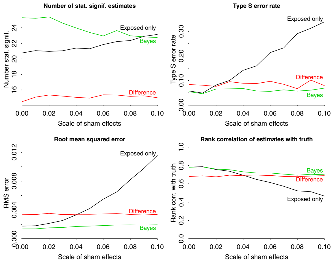
FIGURE 7 Results of simulation study comparing three estimates—the exposed data estimate, y_{j1} , the difference between exposed and sham, y_{j1} - y_{j0} , and the Bayesian hierarchical model estimate E(\theta_j|y) —to simulated data. The four graphs show the results for four different frequency evaluations, and on each graph the horizontal axis represents \sigma^b , the SD of the sham effects in the simulation [Colour figure can be viewed at wileyonlinelibrary.com ]
