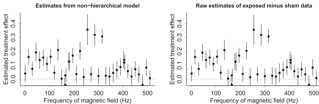
FIGURE A4 A, Posterior mean \pm SD of each treatment effect \theta_j from the nonhierarchical model, which partially pools neither the biases nor the treatment effects, as fit to the chick data. B, For comparison, the raw difference estimate y_{j1} - y_{j0} for the chick data \pm standard error. These two estimates roughly coincide
