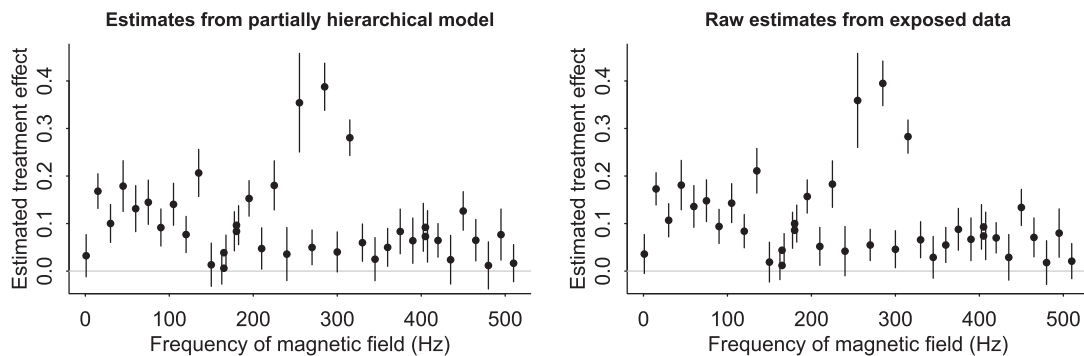
FIGURE A3 A, Posterior mean \pm SD of each treatment effect \theta_j from the partially hierarchical model, which partially pools the biases but not the treatment effects, as fit to the chick data. The fitted model estimated the sham effects to be essentially zero (see discussion of Table 2), and so these estimated treatment effects come pretty much from the exposed data alone. B, For comparison, the raw estimates y_{j1} from the exposed data. These two estimates roughly coincide
