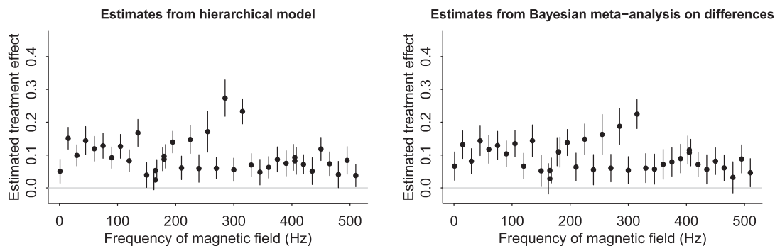
FIGURE A5 A, Posterior mean \pm SD of each treatment effect \theta_j from our proposed hierarchical model that separately models treatment and sham effects. B, For comparison, the estimates given by a Bayesian meta-analysis in the sense of a hierarchical model for the difference estimates
